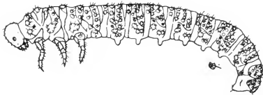
Fig. 95. Imported currantworm, Pteronidea ribesii (Scopoli).
